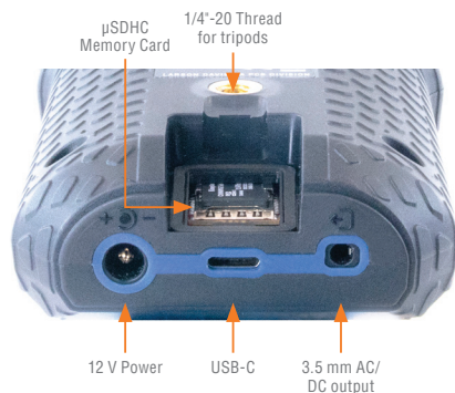
Meter Ports
