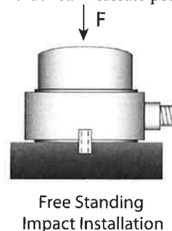
Figure 3 - Series 200 ICP® Impact Sensor
