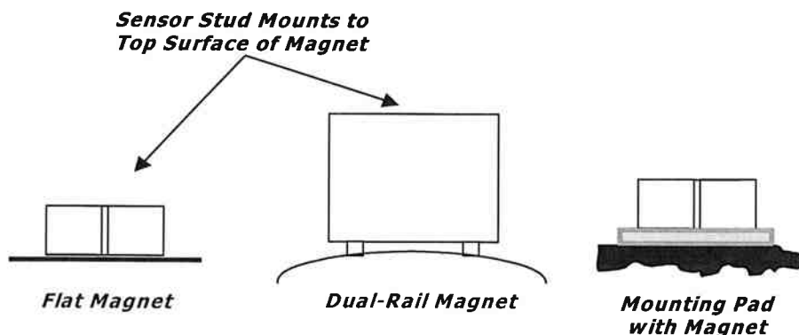
Figure 9 – magnet types
