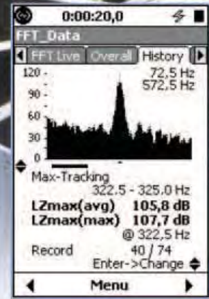
Fig. 27 FFT Max-tracking on Model 831
