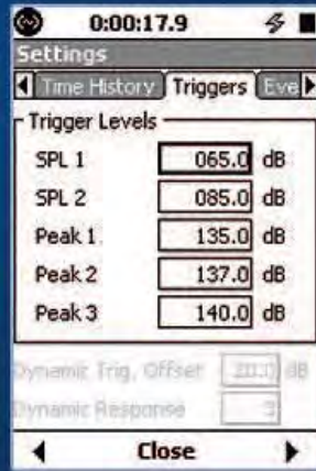
Fig. 4 Trigger Levels
