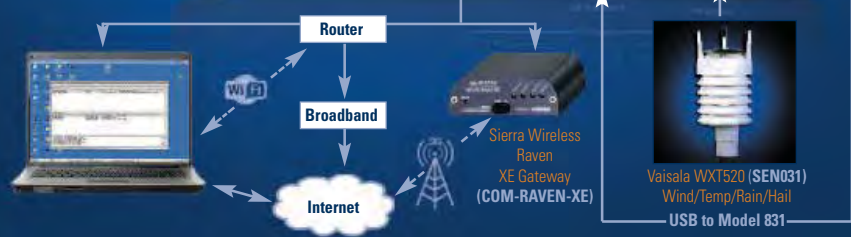
Fig. 9 Model 831-INT Docking Station – Configuration
