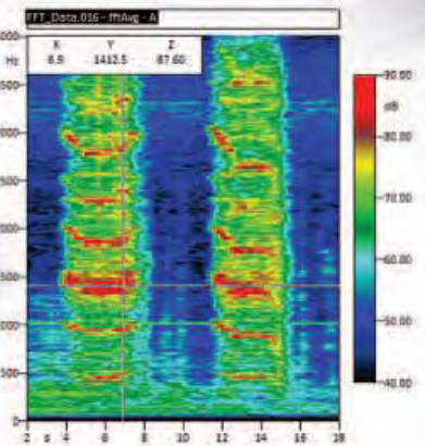
Fig. 28 DNA Software FFT-spectrogram of Stone-cutting Operation
