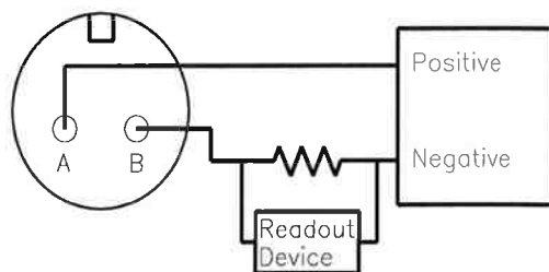
Figure 2 – wiring: loop powered/DC source
